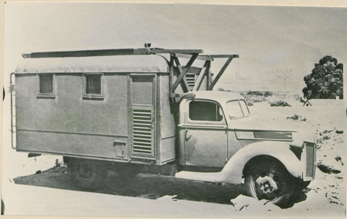
J. B. 5. MOBILE - PACKED FOR TRAVELLING.
