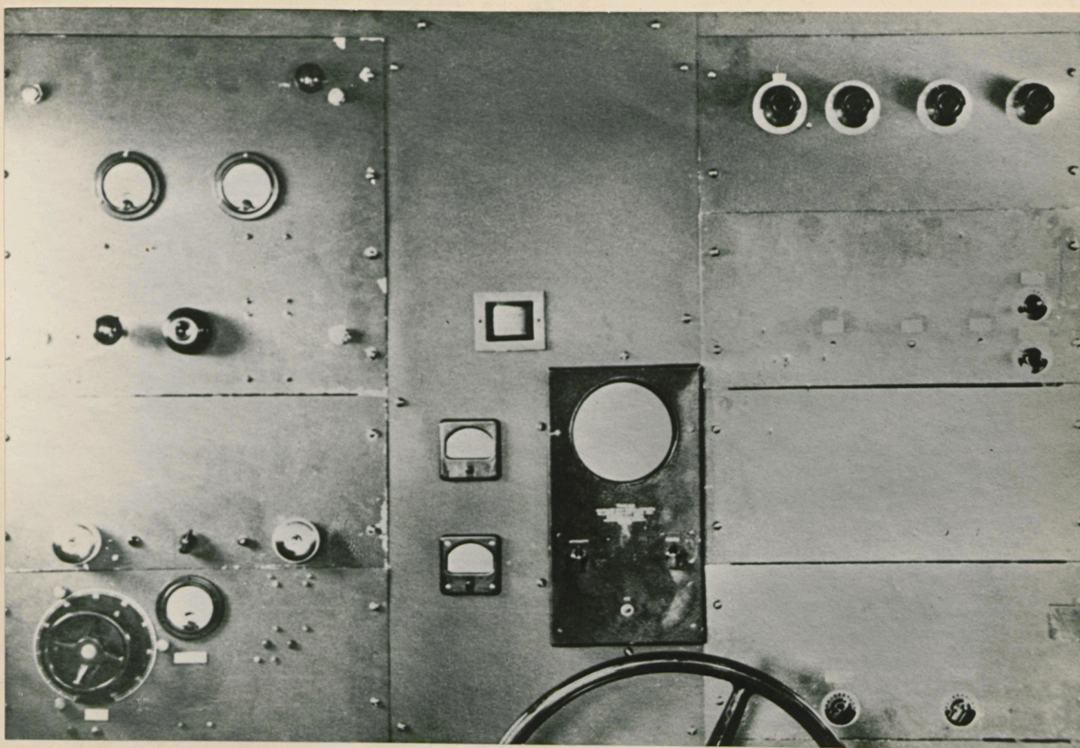
J. B. 5. TRANSMITTER, RECEIVER AND DISPLAY COMBINATION.
